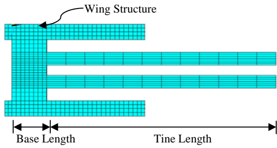
Fig. 7, Tuning Fork Type A
