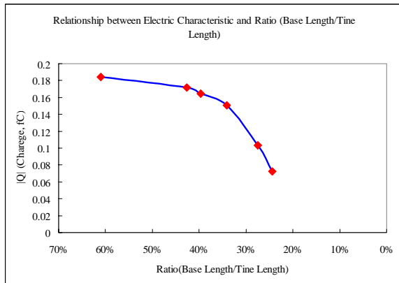
Fig. 4, Relationship between Electric Characteristic and Ratio (Base Length/Tine Length)
