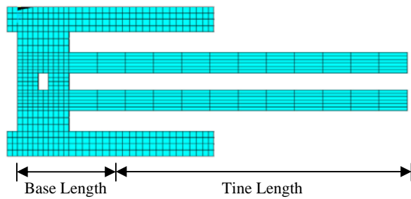
Fig. 8, Tuning Fork Type B
