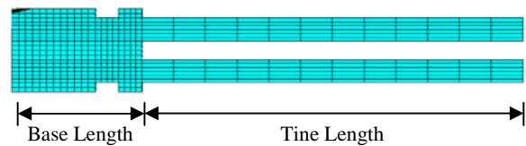
Fig. 6, Modified Tuning Fork with Notch
