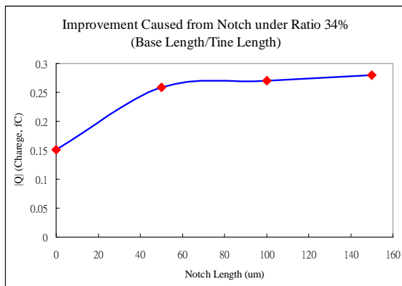
Fig. 5, Improvement Resulted from Notch under Ratio 34% (Base Length/Tine Length)
