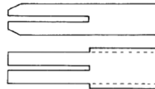
Fig. 2, Modified Tuning Fork with arm corners cut off and base-width [5]
